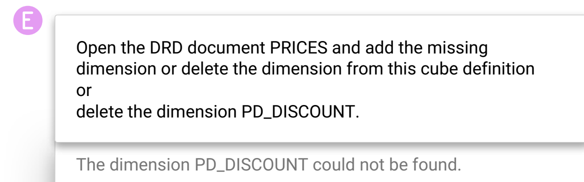
User Action, details
