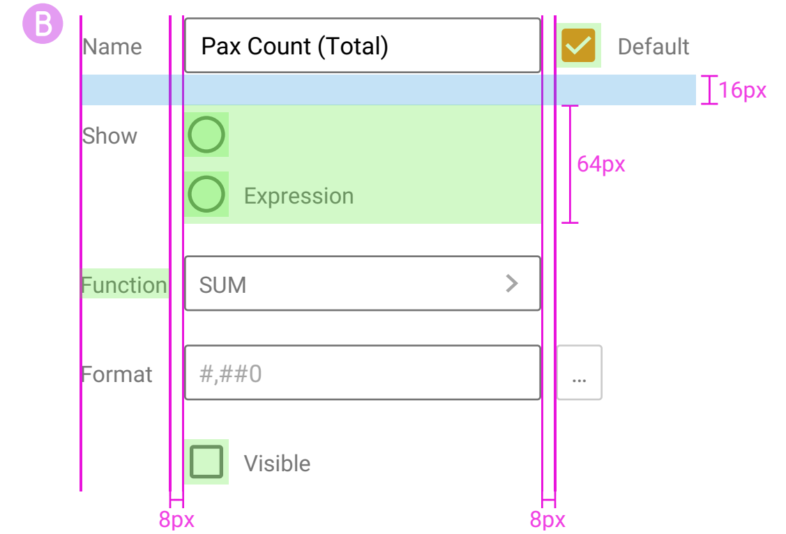
Rule Alignment and Spacing, Vertical
