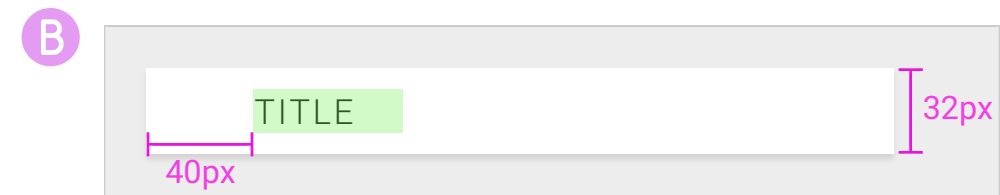
Navigation Search Field, default
