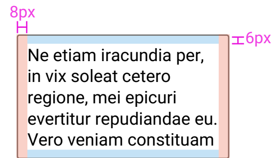
Internal, Text area Field
