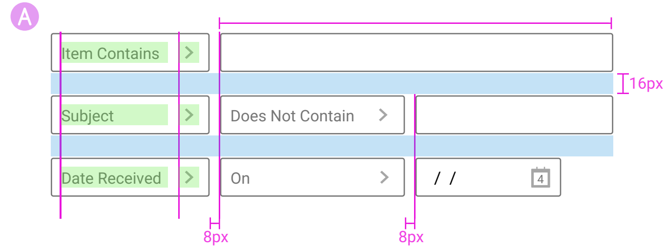
Rule Alignment and Spacing, Horizontal
