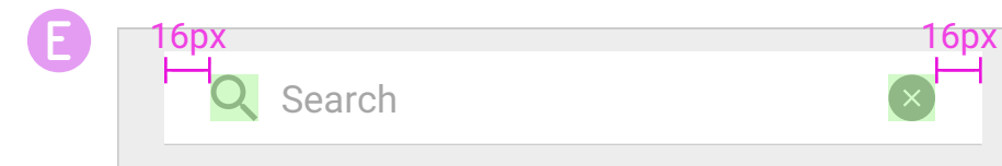
Navigation Search Field, active
